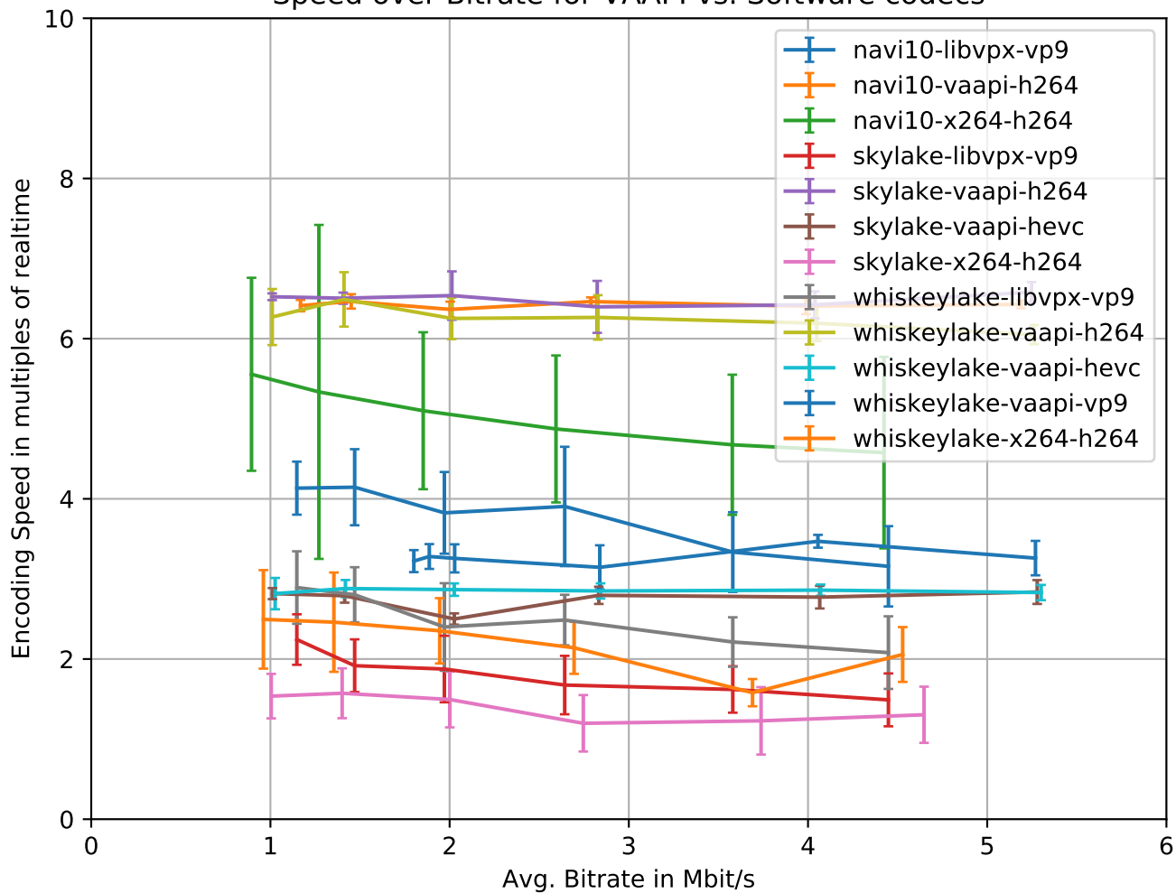
Speed over Bitrate for VAAPI vs. Software codecs
