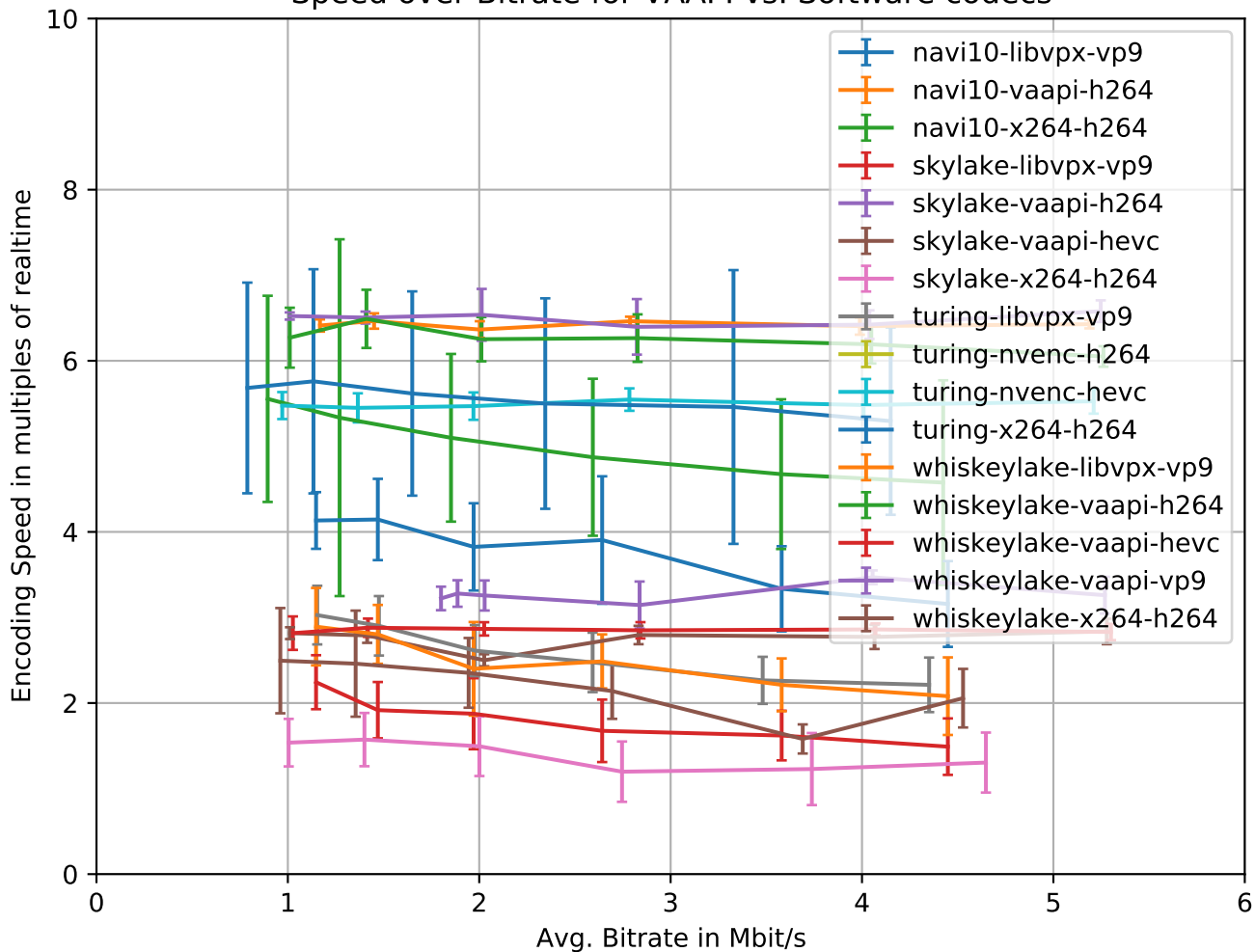
Speed over Bitrate for VAAPI vs. Software codecs
