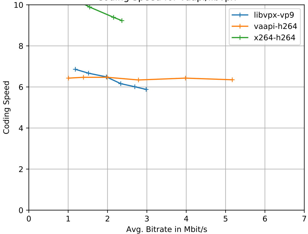
Coding Speed for vaapi/libvpx
